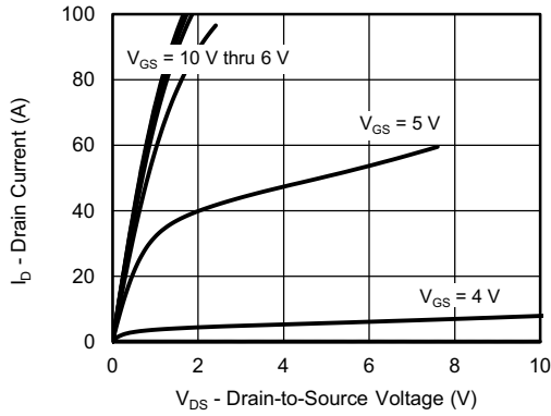
Output Characteristics
