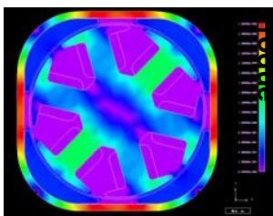
Magnetic Field
