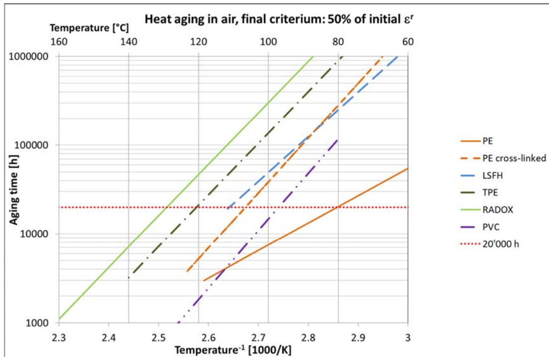
Figure 2: Arrhenius plots for some polymers used in coaxial cables.
